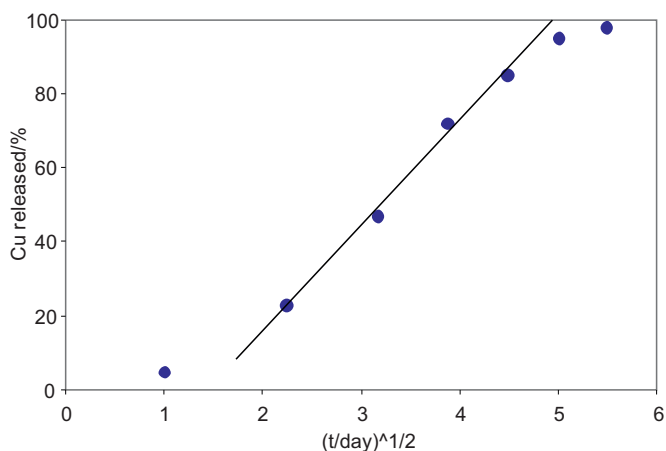
Figure 5. Higuchi diagram of copper release from alginate/chitosan capsules
