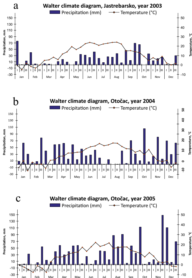
Graph 1 (a, b and c). Walter climate diagrams for meteorological stations Jastrebarsko and Otočac
